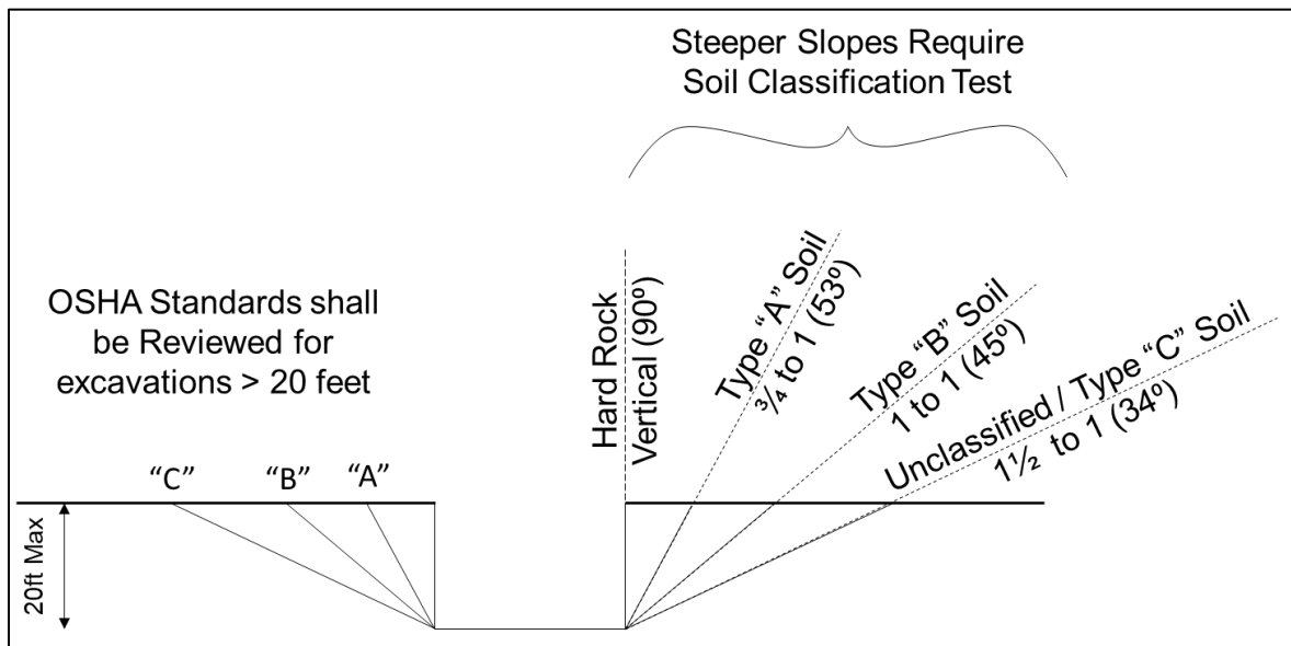
Figure 6 Minimum Acceptable Excavation Design Profiles and Angles
